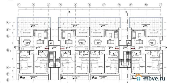
PLAN First Floor
