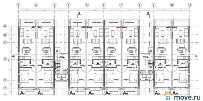
PLAN Ground Floor
