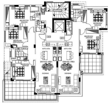
3rd floor
