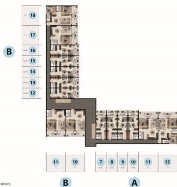
LEMON APARTMENTS FIRST FLOOR PLAN BLOCK A-B
